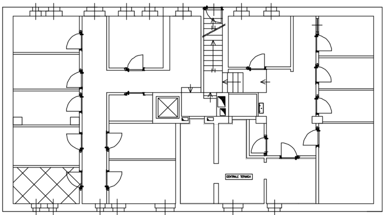
PIANO INTERRATO
