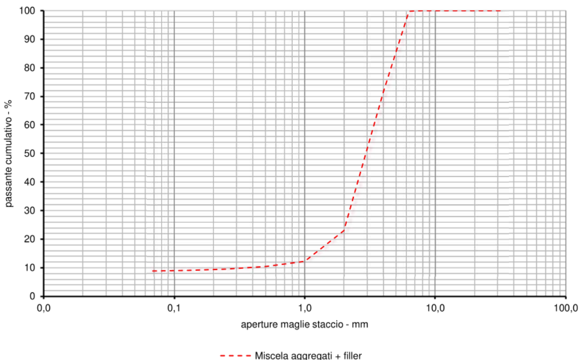
Curve granulometriche
