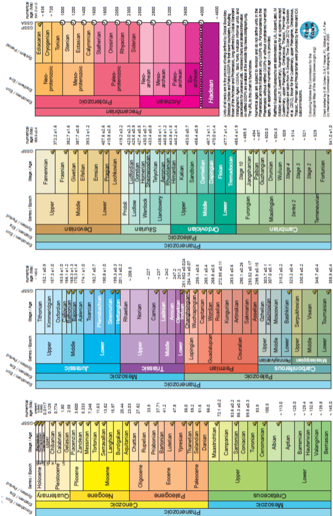
Figura 10. Scala geocronologica (INTERNATIONAL CHRONOSTRATIGRAPHIC CHART da www.stratigraphy.org )
